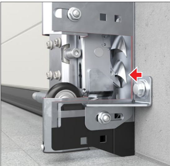
The locking hook of the anti-lift kit automatically latches if the door is forced upwards.
