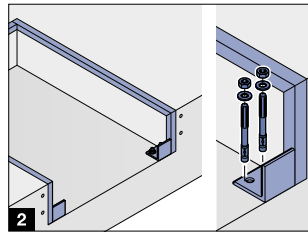
Rear view of pit model P, delivery including lifting equipment
