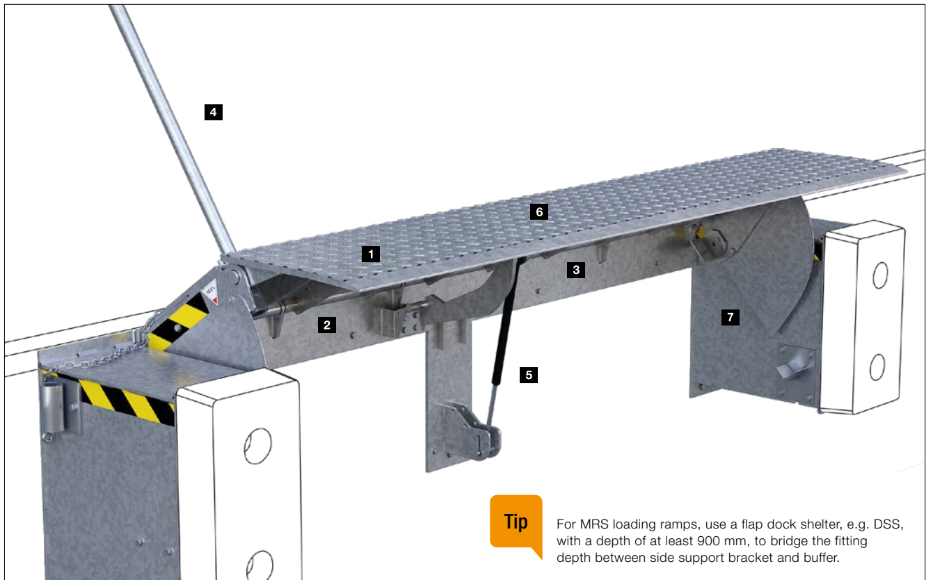
Mechanical dock leveller MRS-V in galvanised version
