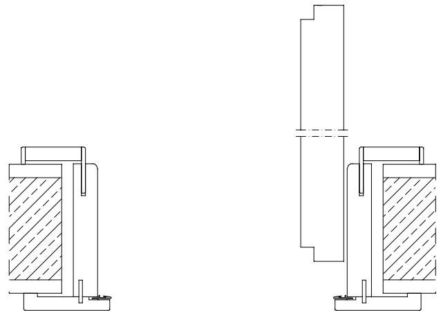
Open (Left-hand hinged)
