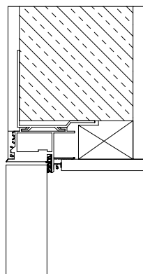
Horizontal sectional view with flush-closing door
