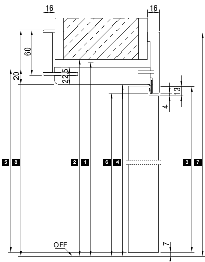
Vertical view
