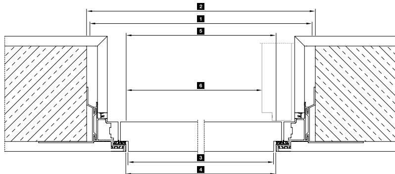
Horizontal view with reverse-opening door leaf
