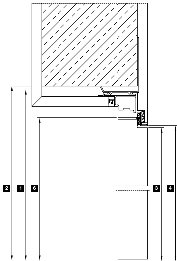
Vertical view with reverse-opening door leaf
