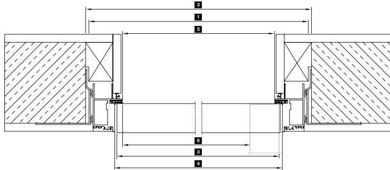
Horizontal view with flush door leaf
