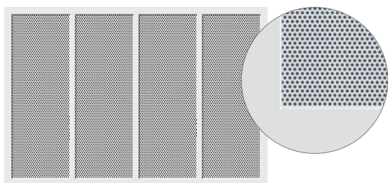
Styles 412 and 432 Internal perforated sheet infill (Style 412 perforated steel sheet, style 432 perforated aluminium sheet) with round recesses, ventilation cross-section 46.1%
