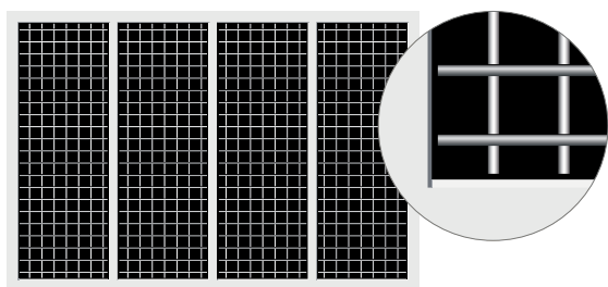
Style 403 Welded grille infill on the inside, ventilation cross-section 85%
