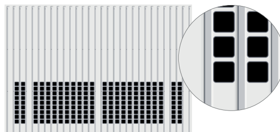
NEW. Style 414 (ET 450) Surface-mounted, ribbed sheet steel with square perforation 50 x 50 mm in the bottom or top section (Fig. shows bottom section), ventilation cross-section 11.5%.
