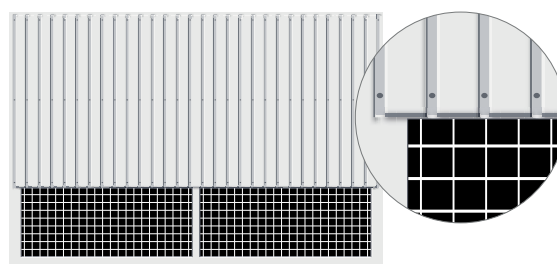
NEW. Style 416 (ET 450) Surface-mounted, ribbed sheet steel with 50 x 50 mm mesh infill in the bottom or top section (Fig. shows bottom section), ventilation cross-section 23.2%
